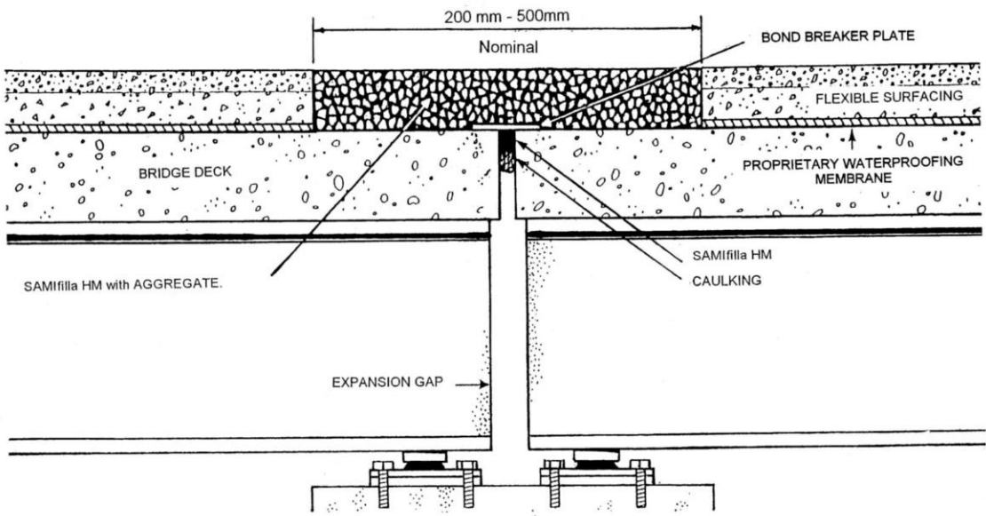
Typical Section Through Bridge Joint SAMifilla Bridge Joint System
